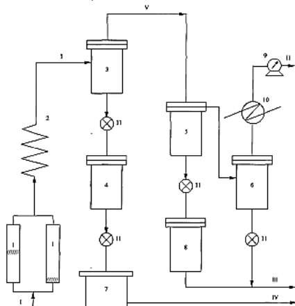
Figure 1 – Schematic diagram of a pilot plant for the thermochemical processing of heavy oil residues
